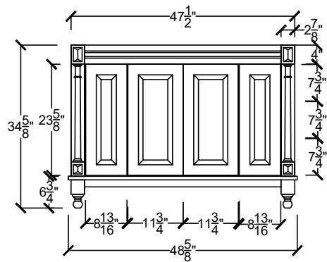
LEXV 4822 - - - - CENTER BOWL SINK
