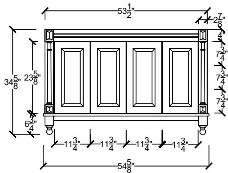
LEXV 5422 - - - - CENTER BOWL SINK
