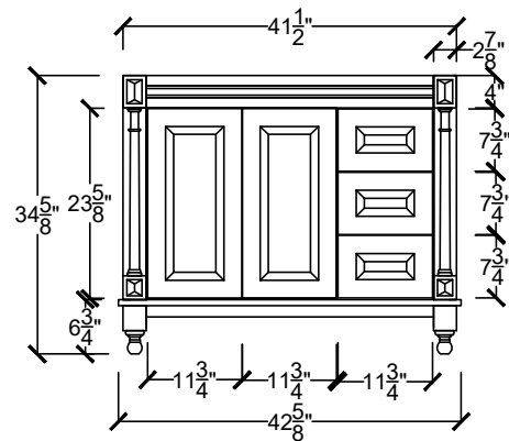
LEXV 4222 3DL OR 3DR- _ _ _
