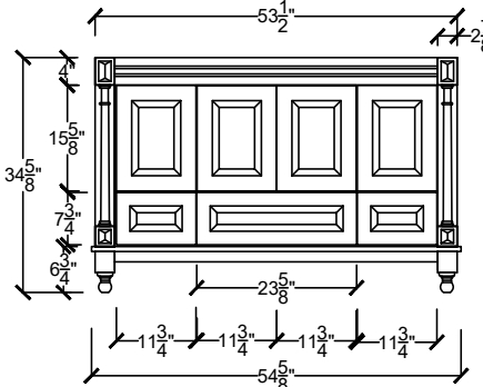
LEXV 5422 BD- - - - CENTER BOWL SINK
