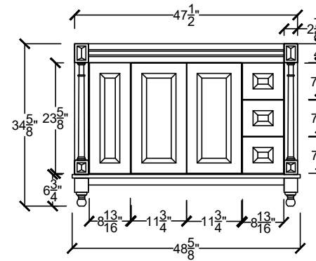
LEXV 4822 3DL OR 3DR- - - -
