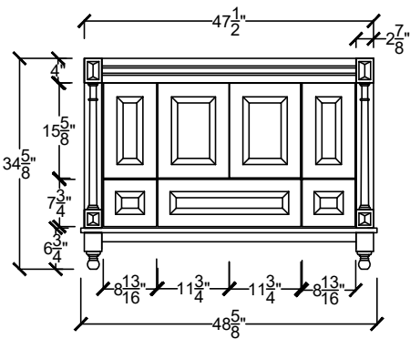
LEXV 4822 BD- - - - CENTER BOWL SINK
